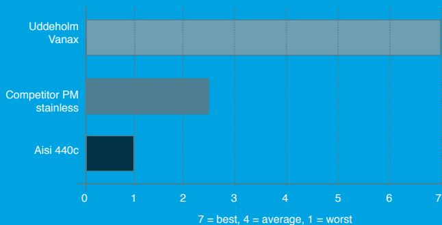
Corrosion resistance
